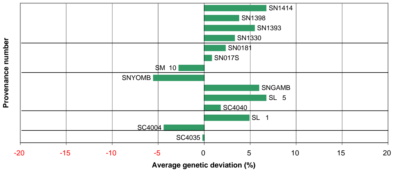
Landraces - Pilodyn measure at late evaluation (overall average = 12.3 mm)
